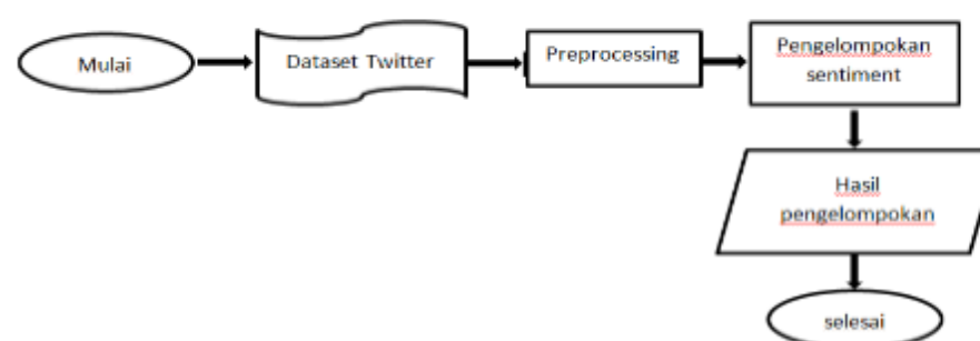
Gambar 1. Flowchart penelitian
