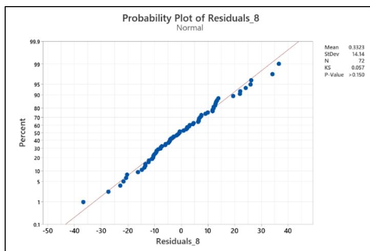
Gambar 4. Plot Uji Normalitas Residual ARIMA(4, 0, 4)(0, 1, 0)^{12}
