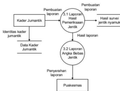
22 Gambar 7 Data Flow Diagram (DFD) level 2 Pelaporan
