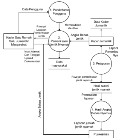
2 Gambar 4 Data Flow Diagram Level 1
